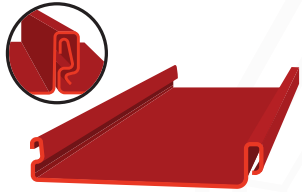
1.5" Snap Lock Standing Seam
