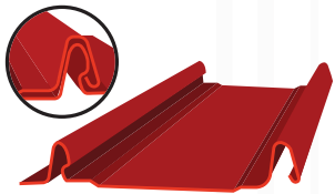
1" Snap Lock With Slotted Flange AKA 1" Nail Strip
